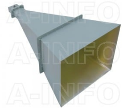
LB-430-20-C-SF Standard Gain Horn Antenna 1.7-2.6GHz 20dB Gain SMA Female
